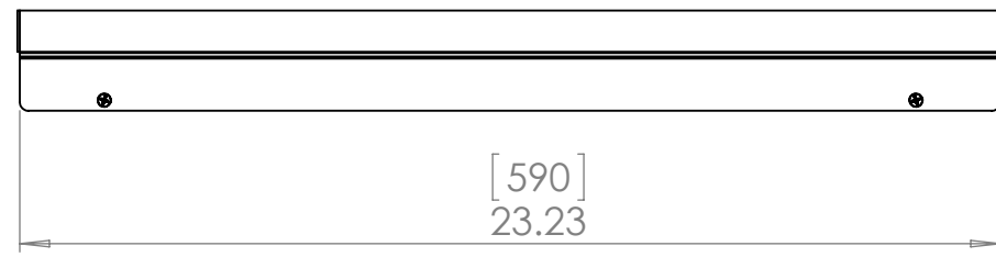
3800.24.LP Vaya Linear MP Louver, 24in
